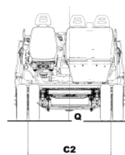
Rear view
